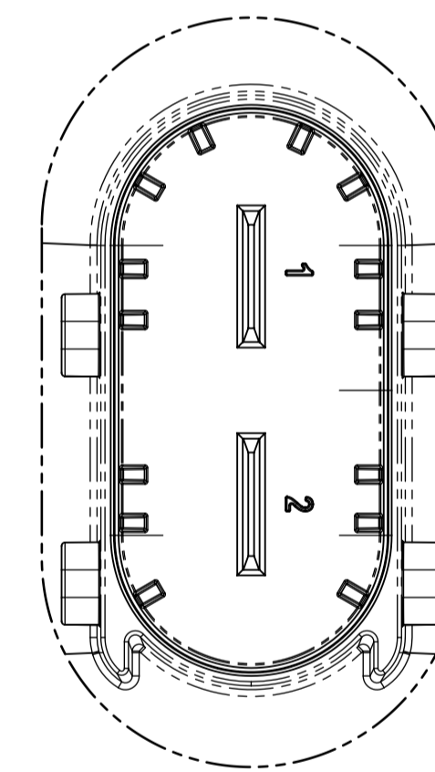
DETAIL D SCALE 2 : 1
