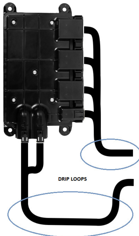
IX3212 PDM shown in preferred mounting orientations
