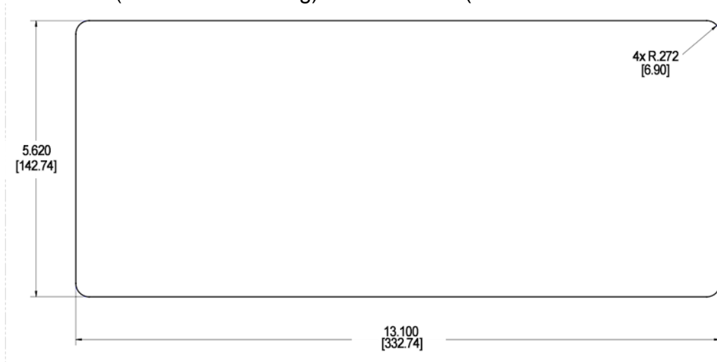
RECESSED MOUNT PANEL CUTOUT DIMENSIONS FULL SCALE
