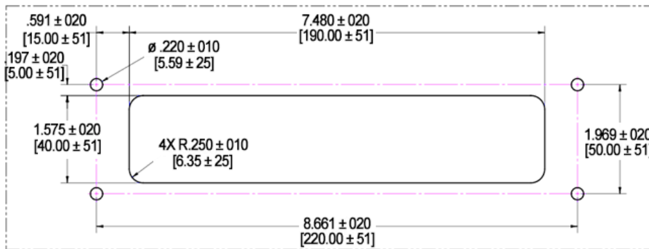
SURFACE MOUNT PANEL CUTOUT DIMENSIONS FULL SCALE
