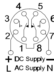
Relay shown de-energised
