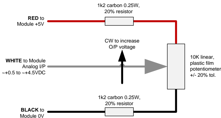
Equivalent DC electrical circuit:
