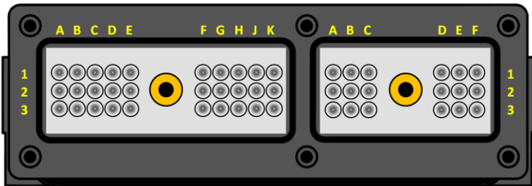
↑ 30 Way Metri-Pak Connector
